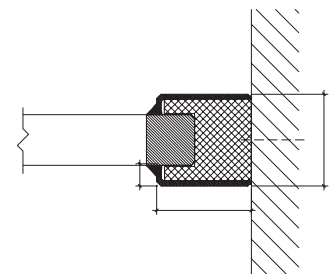
Wall connection
