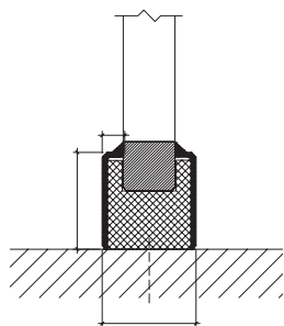
Floor connection
