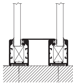
Ceiling connection
