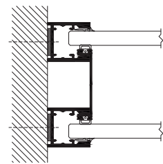
Wall connection
